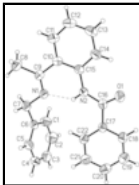
Fig. 1. A view of the molecular structure of I with the atom numbering scheme. Displacement ellipsoids are drawn at the 30% probability level. H atoms are presented as a small spheres of arbitrary radius. Intramolecular H-bond drawn by dashed line.
